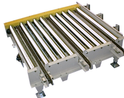
SCAMBI A 90 GRADI / EXCHANGES AT 90 DEGREE
